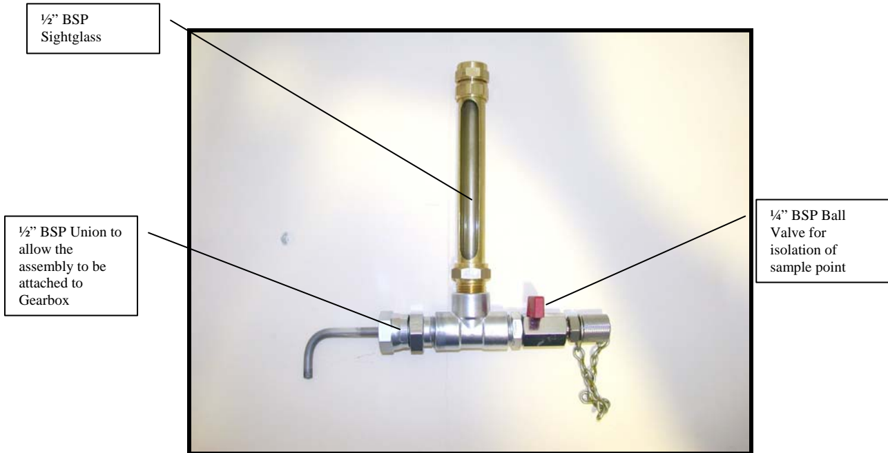
Sight Glass and Sample Point Assembly Examples Only
